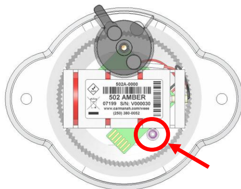
Figure 2. Location of Vent (Switched Model 502 Shown)
