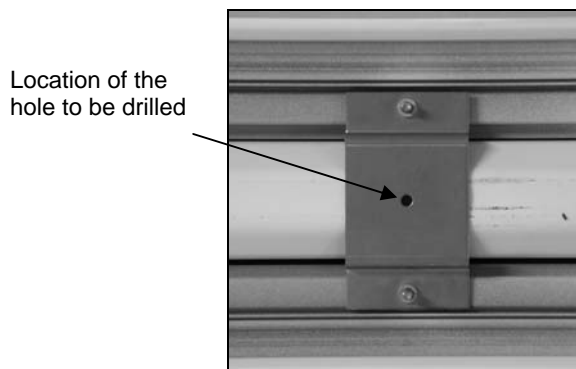
Figure 10: Bracket Detail
